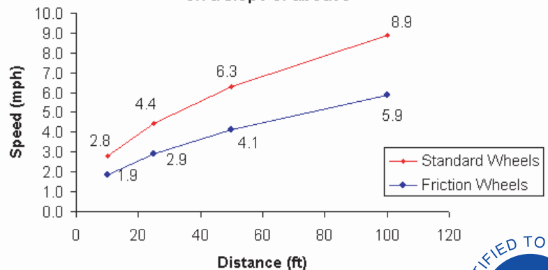
Relationship between distance and speed on a slope of about 5°
